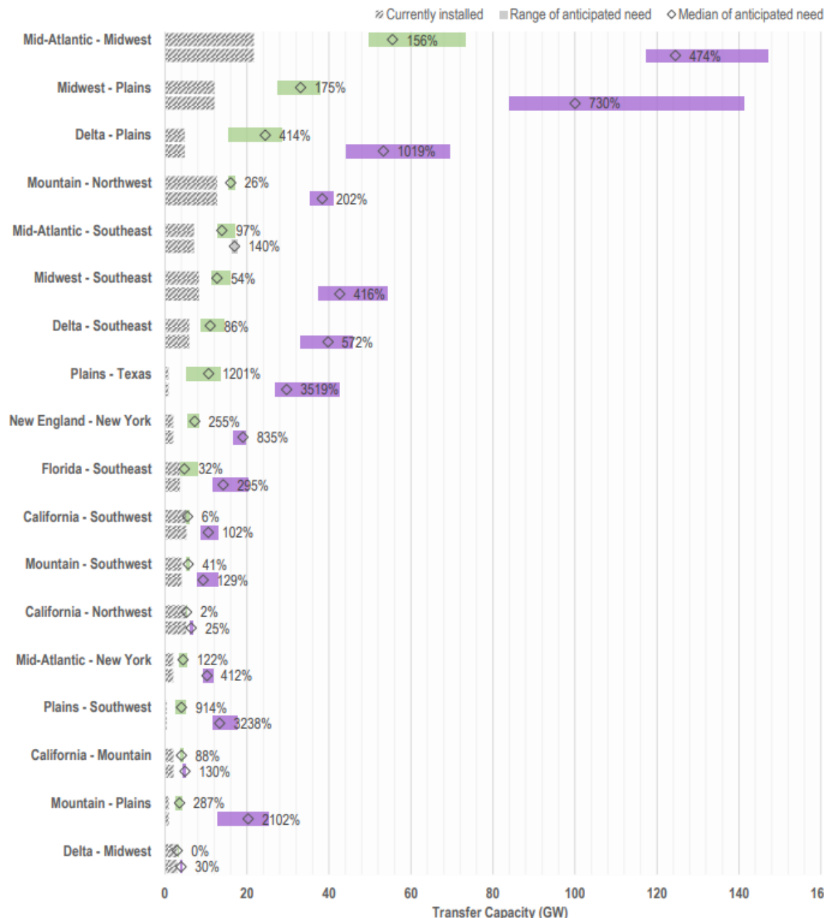
Anticipated interregional transfer capacity need in 2035 for two scenario groups Range of new transmission need for future scenarios with moderate load and high clean energy growth (green, top for each region pair) and high load and high clean energy growth (purple, bottom). Median % growth compared to 2020 system shown.
